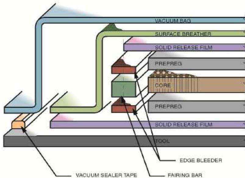
Figure 1: CYCOM 970 Typical Sandwich Layup/Bagging
