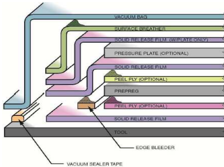
Figure 2: CYCOM 970 Typical Laminate Layup/Bagging
