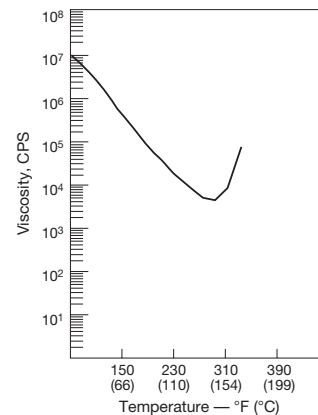
Rheometrics Curve of F155 Resin 4°F (2°C)/min, 10 rad/sec, RDS-7700, 50 mm Plates
